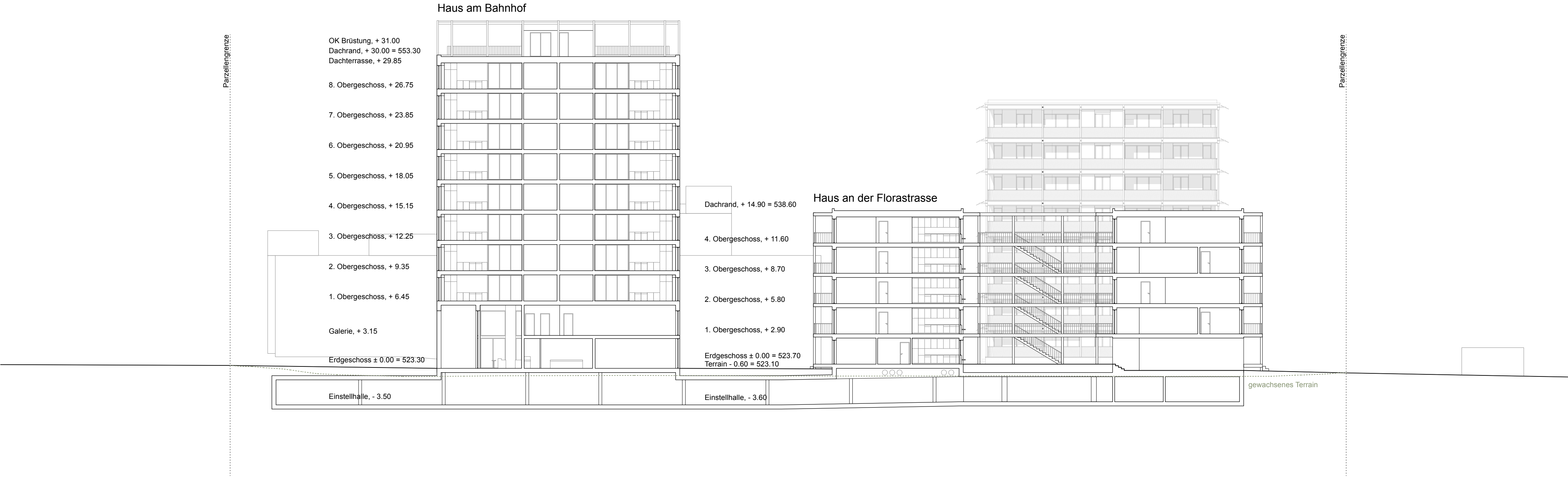
Schnitt Ost-West
